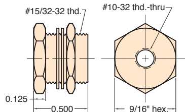
#10-32 Bulkhead Fitting
